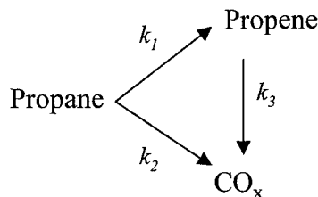
SCHEME 1. Reaction network in oxidative dehydrogenation of propane reactions.
